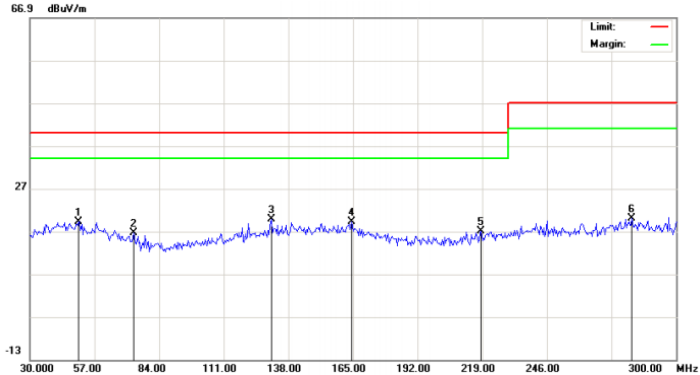
Radiated Emission Test at 3m Distance-Horizontal
